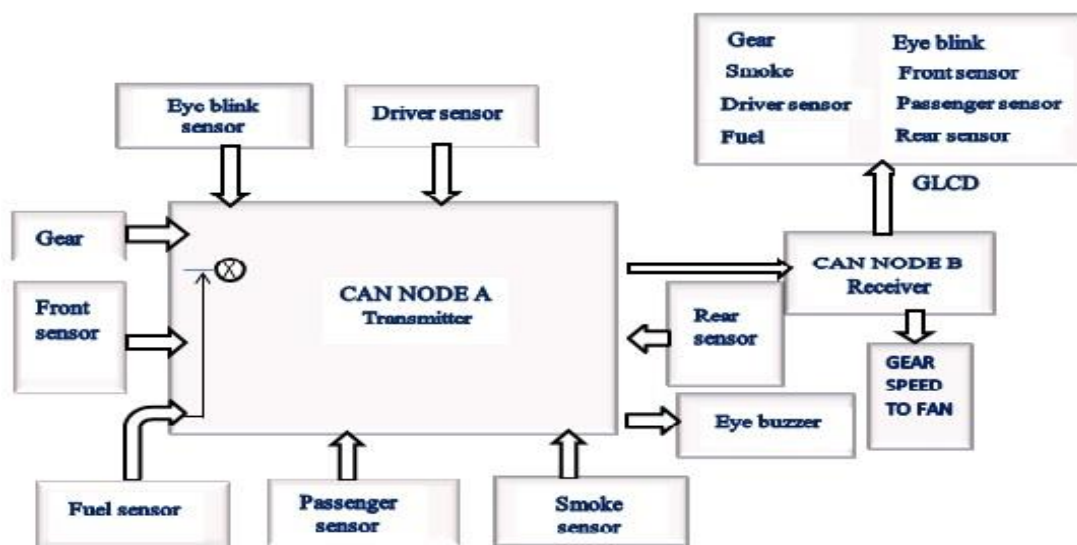
Fig: 1. Block diagram of alerting system
